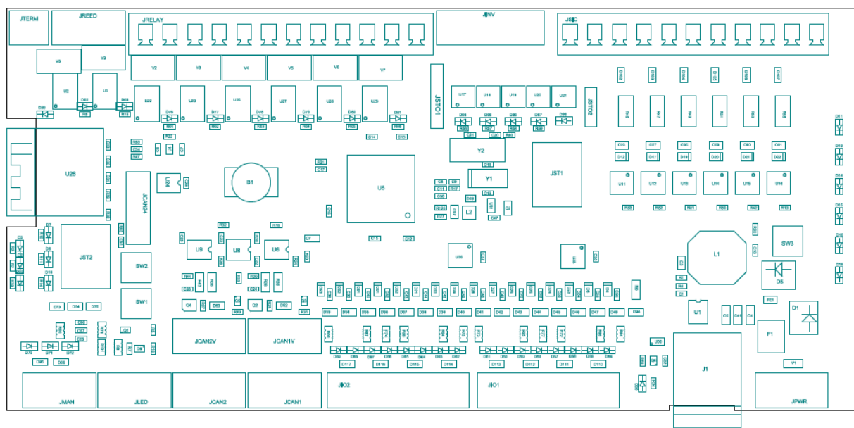
PCB layer: assembly drawing top Rev A – EC 07
